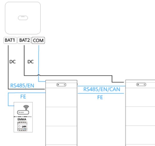
Figure 2-10 Connecting the ESSs to the inverter (2)
