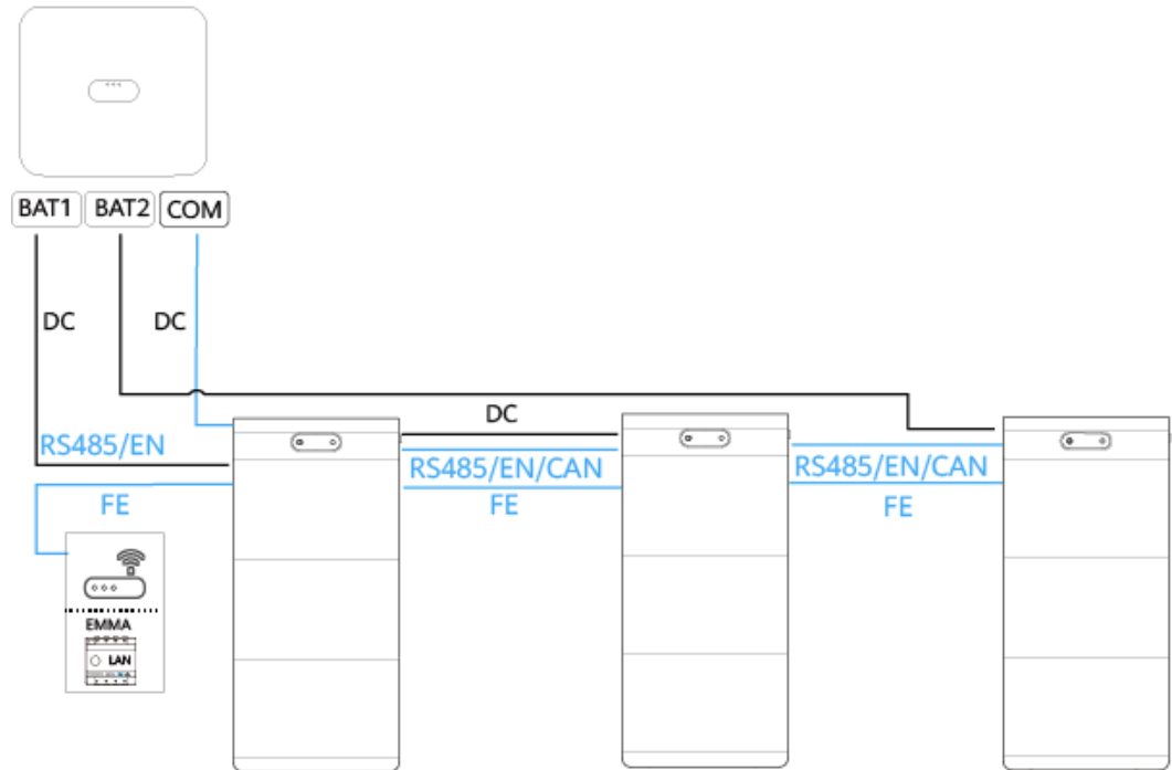
Figure 2-11 Connecting the ESSs to the inverter (3)
